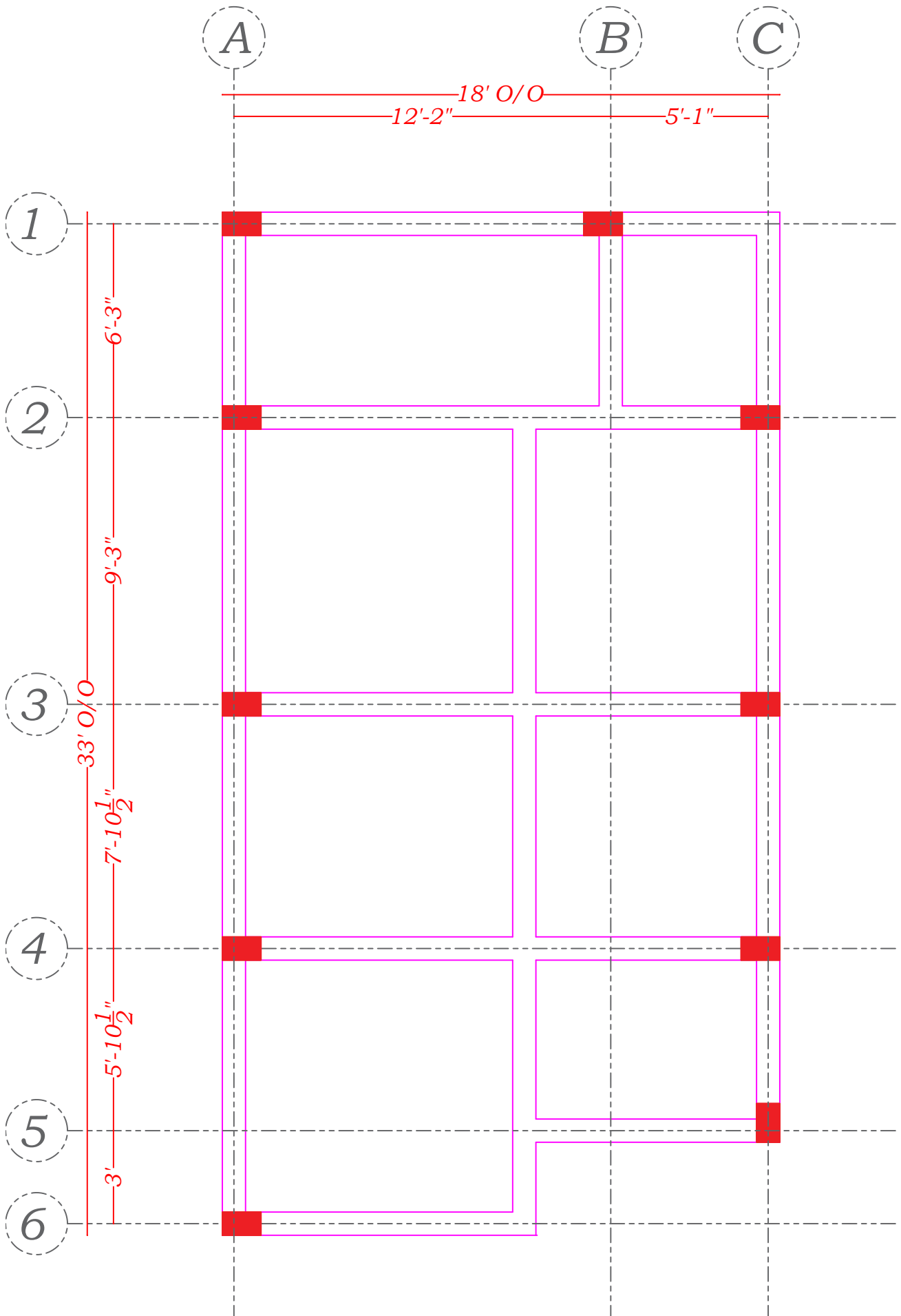
PLINTH BEAM LAYOUT
