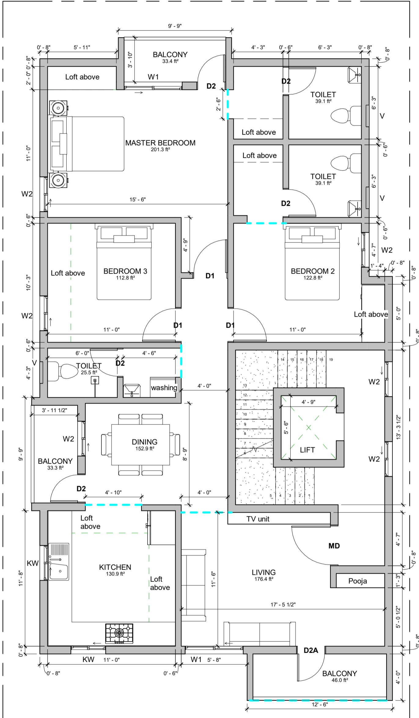
2 FIRST FLOOR LEVEL 1 : 55
