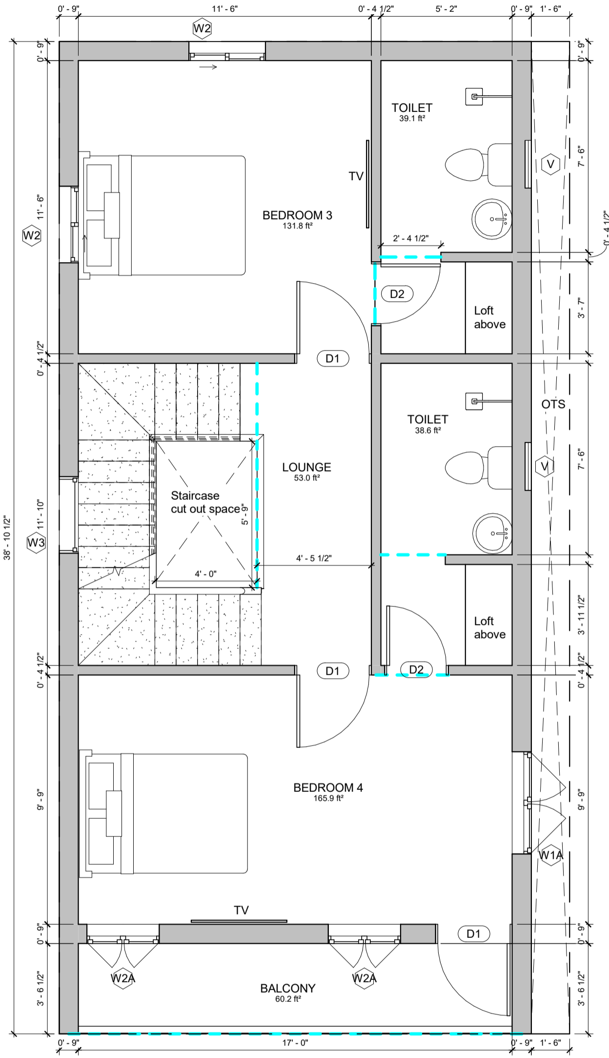
3 SECOND FLOOR LEVEL 1 : 40
