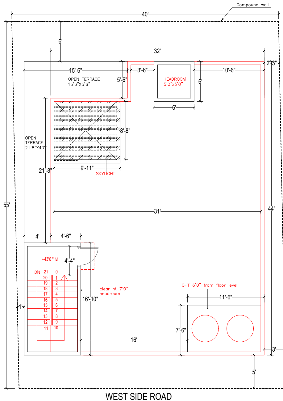
TERRCE FLOOR PLAN
