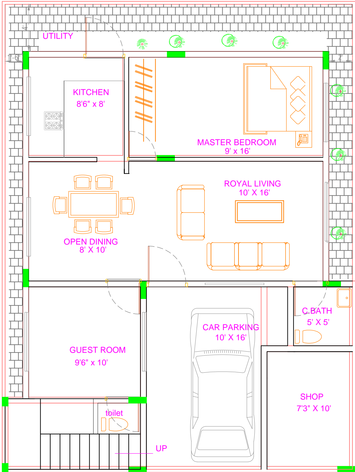
GROUND FLOOR TENTATIVE BEAM AND COLUMN LOCATION
