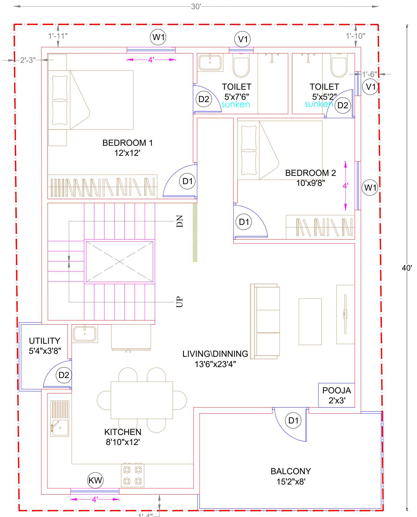
TYPICAL FIRST & SECOND FLOOR PLAN
