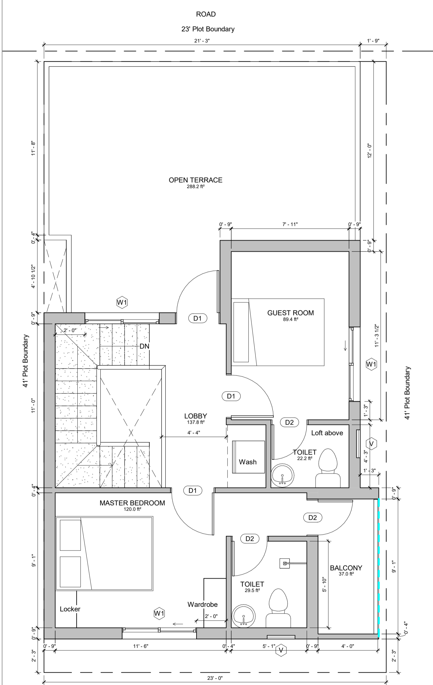
2 FIRST FLOOR LEVEL 1 : 40
