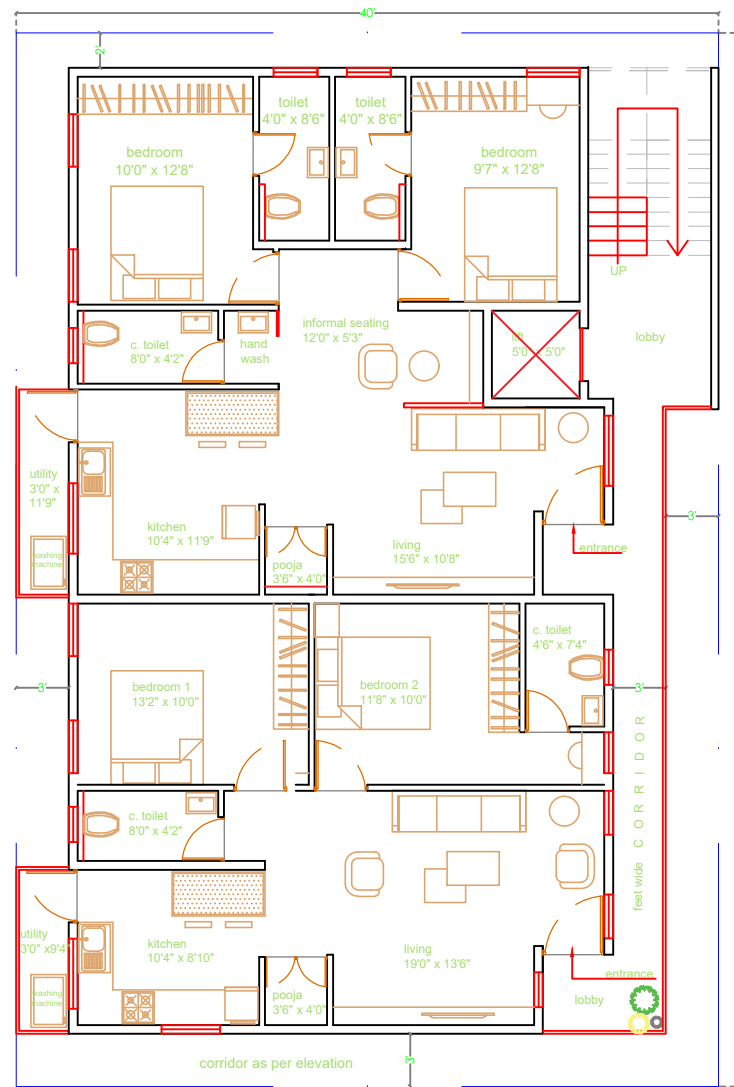
Second floor plan builtup : 1788 sft lobby : 140 sft utility : 65 sft
