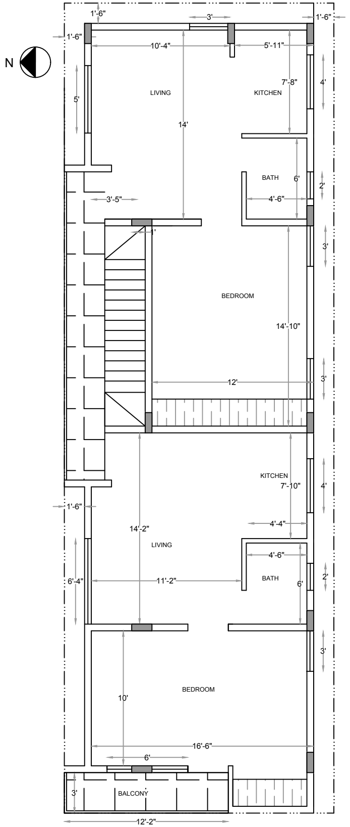
TYPICAL FLOOR
