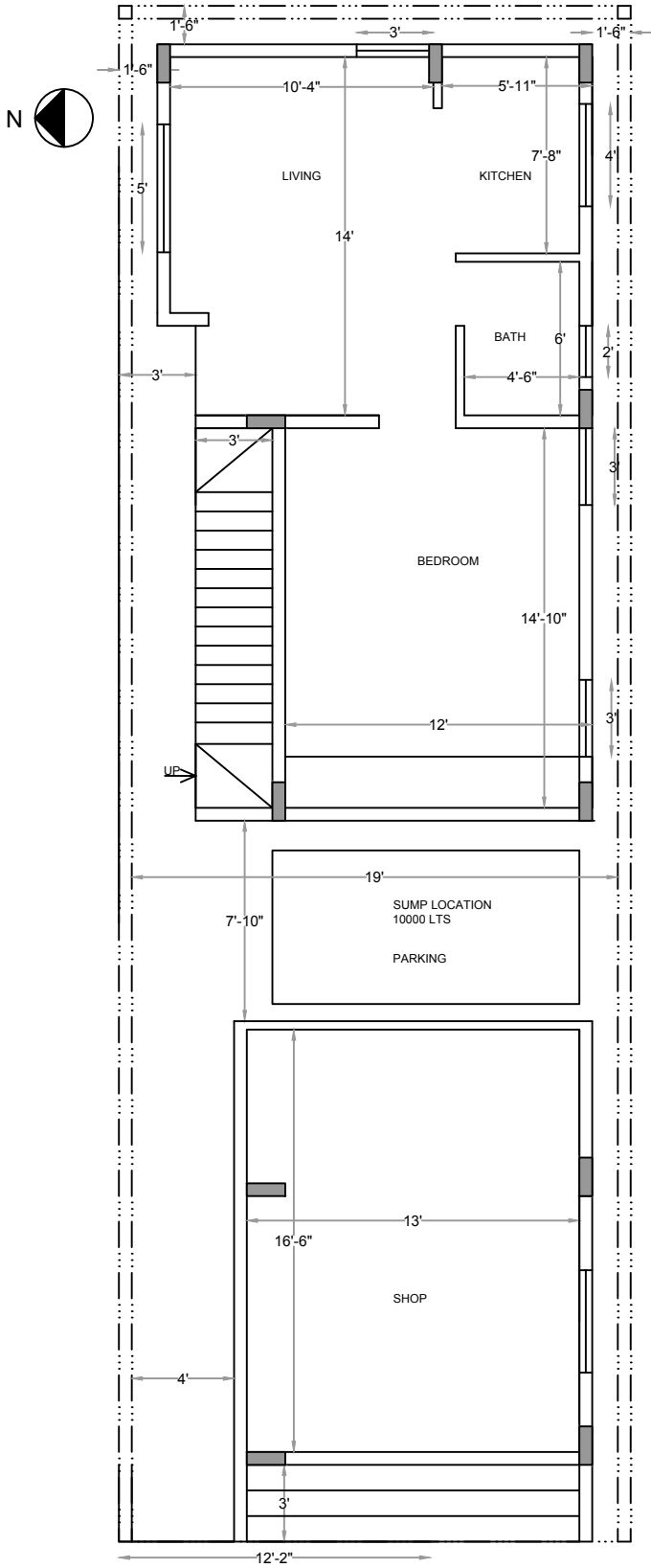
GROUND FLOOR
